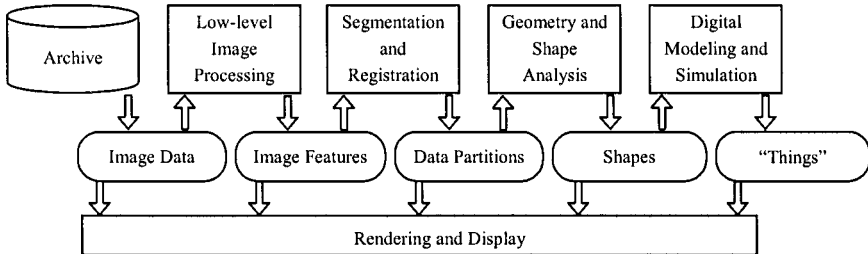
Figure 12-3. An idealized view of the medical visualization pipeline. This part of 3D Informatics encompasses the study the process of medical visualization by research in the four core areas of Volume Image Archives, Low-level Image Processing, Geometry and Shape Analysis, and Digital Modeling and Simulation. Note that the results of many of the subfields can be directly rendered, revealing the information that is hidden within the dataset at different levels of abstraction. One attribute of any informatics program is the progressive abstraction of volume information from image to model.
